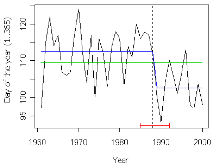
Fig. 1 – Climatic change of '80 years seen analysing the date of leaf unfolding in Germany (data from Chmielewski F.M., Rotzer T., 2001). The analysis, carried out with struchange library of R software, show that the breakpoint drops between 1985 and 1992 with a confidence of 90% and that the most probable year of breakpoint is 1988; the mean date was 112.5 before and 102.5 after the breakpoint.
