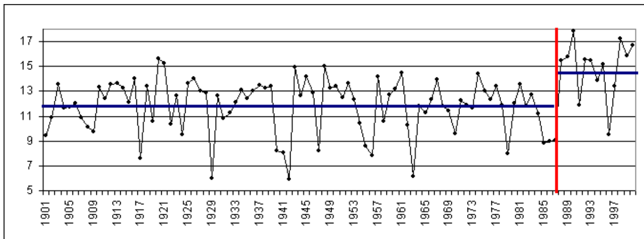
Fig. 2 – Behavior of mean temperature of the first 150 days of the year at De Bilt (Nederlands), a very significant site because it is located in the “bed” of the westerlies. In 1989 this temperature, almost stationary from 1900 shows an abrupt increase (vertical line in bold) that indicates the beginning of the present climatic phase. The average temperature is of about 12°C for the period before the breakpoint and 14.5 for the period after.
