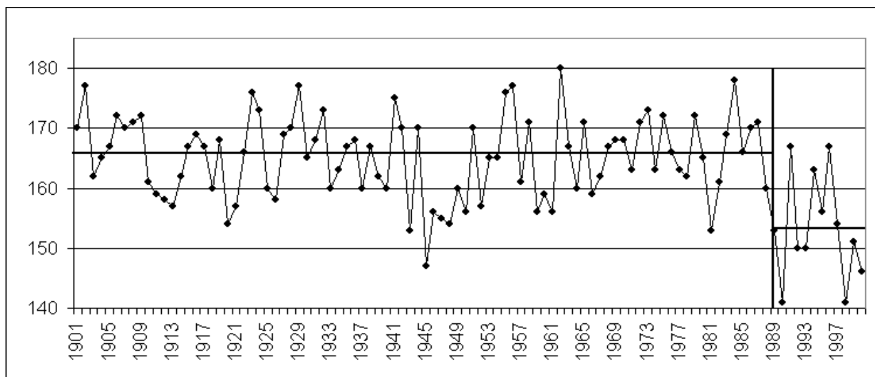
Fig. 3 – Flowering of the black elder ( Sambucus nigra ) at De Bilt (140=20 of may). It is evident the very strict link between temperature and phenology with flowering data that reacts almost immediately to the increase of temperatures. The average date is about 166 before the breakpoint and 153 after the breakpoint, about two weeks of advance (source of data: van Vliet et al., 2002).
