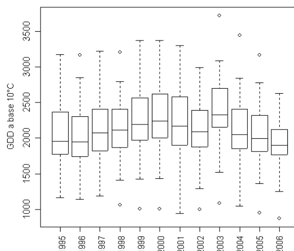
Fig. 5 – Boxplots of yearly growing degree days cumulated on the base temperature of 10°C from the daily data of 90 stations available on Ucea web site (each boxplot represents maximum, upper quartile, median, lower quartile and minimum; outliers are excluded from calculations and represented with circles). A gradual decrease is evident after the high values attained in 2003.
