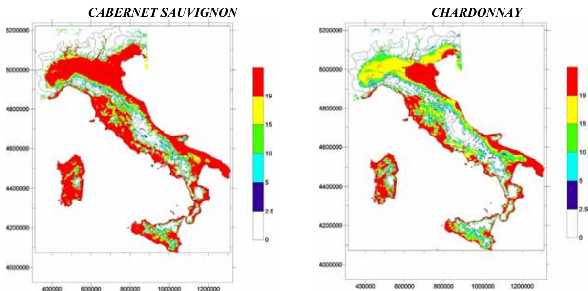
Fig. 4 – Some phenological maps developed by IPHEN project on May 10 th 2006. The maps are obtained with a phenological model based on the summation of the Normal Heat Hours obtained from temperature data of Ucea network. The first guess field was corrected by means of data produced by phenological observers.
