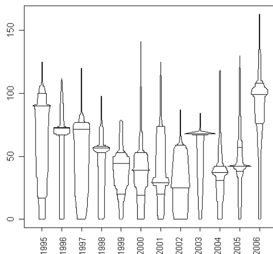
Fig. 6 – Box-percentile plots of date (day of the year) of the last late frost for the 90 stations available on Ucea web site (horizontal lines represent maximum, upper quartile, median, lower quartile and minimum; for more information about the meaning of this kind of plot see Easy and Bafield, 2003). A progressive delay of the last frost can be observed in the last years.
